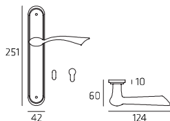
DROPL05P DROPL05Y Maniglia su placca Doorhandle on plate
