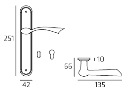
PHEPL05P PHEPL05Y Maniglia su placca Doorhandle on plate
